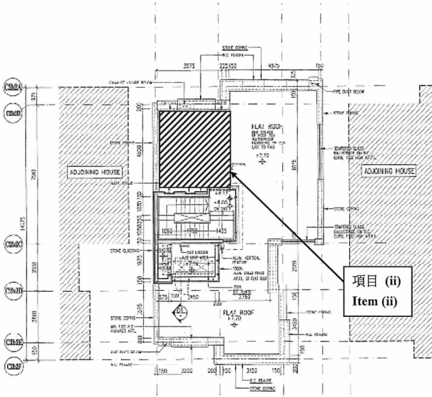
ROOF PLAN - TYPE C2b2 HANDED LAYOUT FOR HOUSE NO.6-7 TO R-13 (REFER DWG. NO. A/CRP31b)
