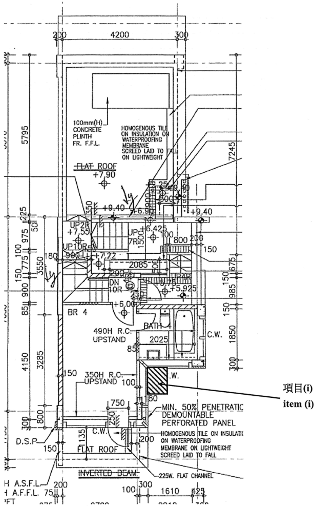
2/F Plan (2 字樓平面圖)
