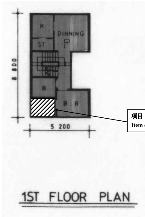
1/F Plan
